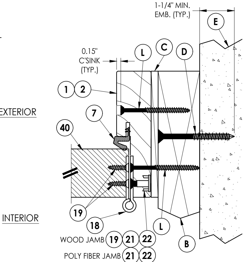
3 HORIZONTAL CROSS SECTION 5 Inswing shown - outswing also approved
