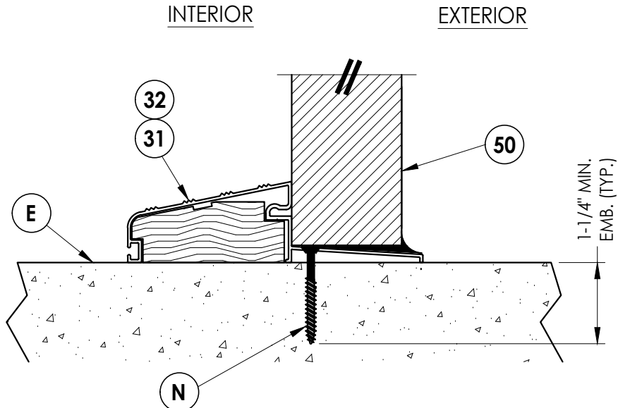
4 8 VERTICAL CROSS SECTION Outswing configuration
